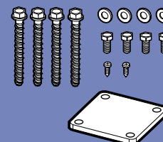
Post Mount Mounting Hardware - Concrete Applications (#1369)
